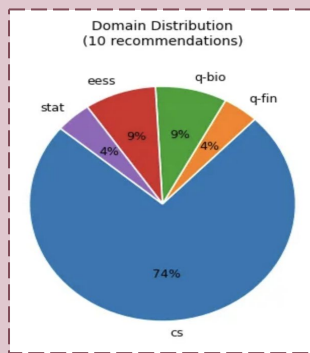
Bandits
